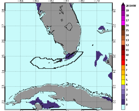
Figure 3. NOAA's Experimental 5km Degree Heating Weeks Map for Florida June 29, 2022. https://coralreefwatch.noaa.gov/vs/gauges/florida_keys.php
