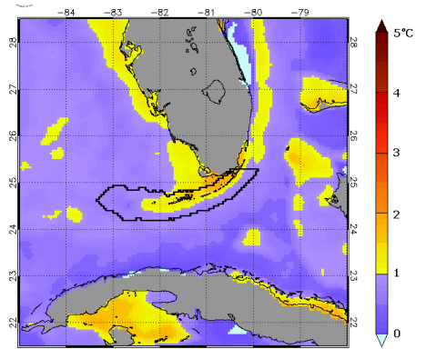
Figure 2. NOAA's Experimental 5km Coral Bleaching HotSpot Map for Florida July 13, 2022. https://coralreefwatch.noaa.gov/vs/gauges/florida_keys.php
