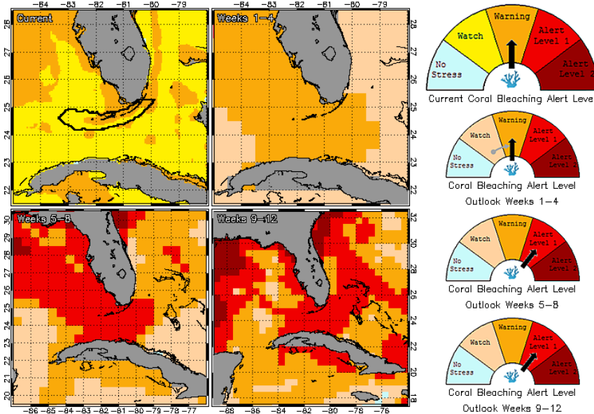
Figure 1. NOAA's 5 km Experimental Current and 60% Probability Coral Bleaching Alert Outlook Areas through October 2022. Updated July 13, 2022. http://coralreefwatch.noaa.gov/vs/gauges/florida_keys.php
