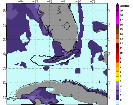
Figure 3. NOAA's Experimental 5km Degree Heating Weeks Map for Florida July 13, 2022. https://coralreefwatch.noaa.gov/vs/gauges/florida_keys.php
